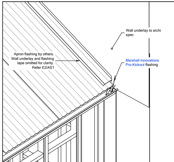
5. Tekton Building Wrap over apron and Pro-Kickout flashing upstands.
