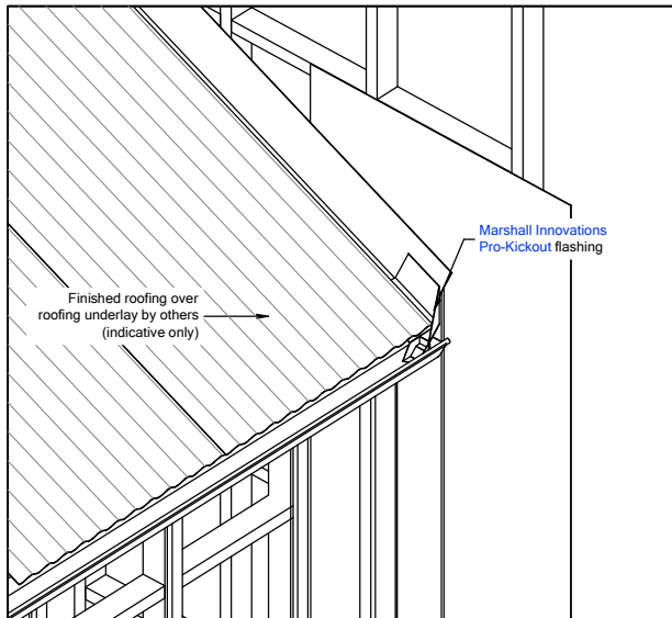
4. Roof cladding system to manufacturer's specifications by others.
