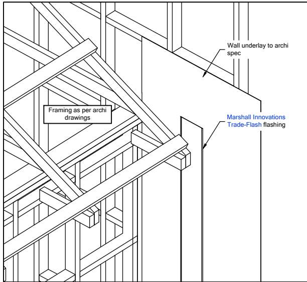
1. Tekton Building Wrap and TRADE-FLASH uPVC back flashing. Supporting structure indicative only.
