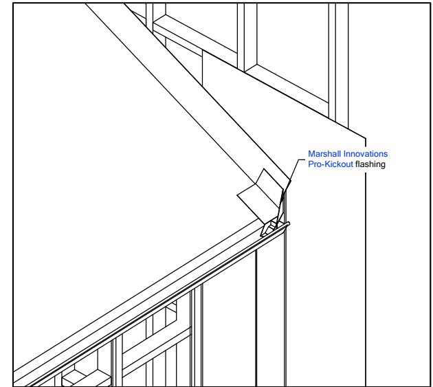
3. Eaves gutter (by others) to stop 10mm clear of finished wall cladding Pro-Kickout Flashing
