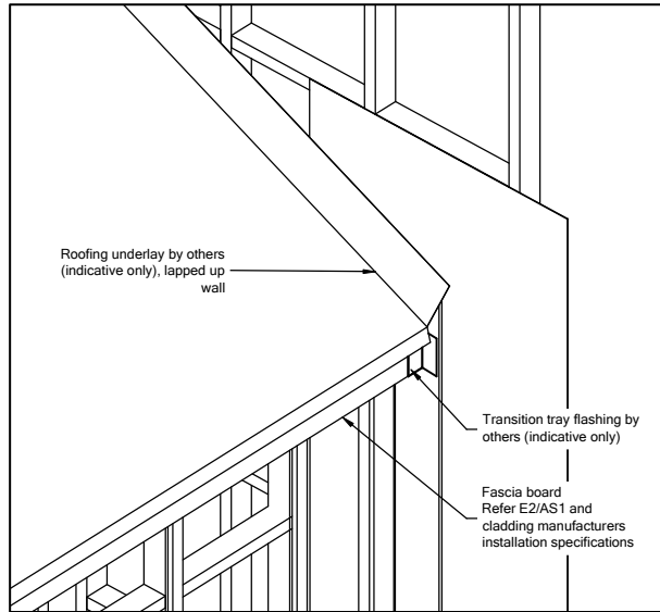
2. Fascia Board Proprietary roofing underlay by others.
