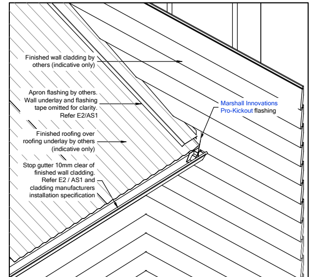
6. Wall cladding system to manufacturer's specifications by others.
